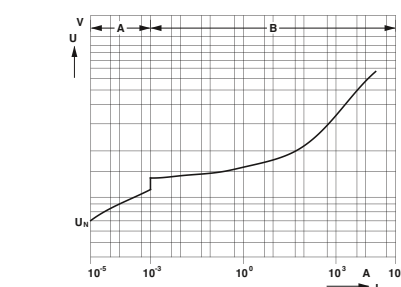
U/I characteristic curve of metal oxide varistors
