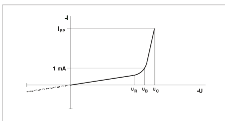
U/I characteristic curve of a suppressor diode
