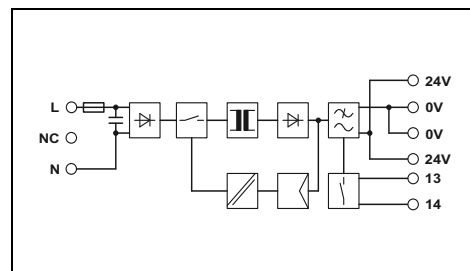
Power supply, 1 AC, 24 V DC, 1.5 A, DIN rail connector optional
