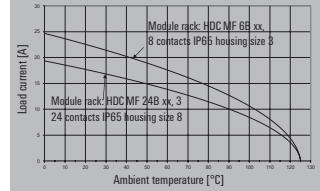
HDC-MHX 4P - modules in IP65 housing / H07V-K6.0 / 8 or 24 poles
